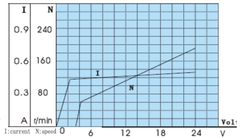
No Load Motor Voltage/Speed/Current/Curve
