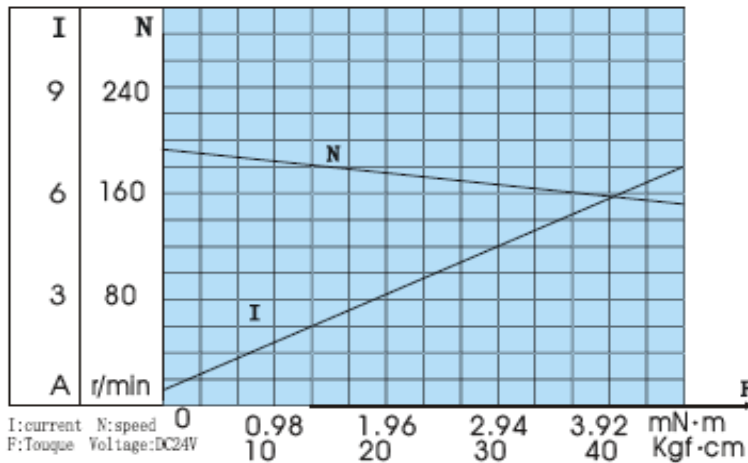
Gear Motor Speed/Current/Torque/Curve
