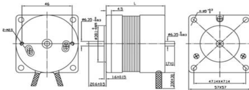
Brushless with square front end bell at 36 rated voltage
