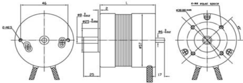
Brushless with round front end bell at 36 rated voltage
